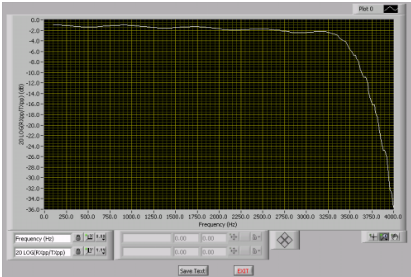
Figure 9. Transhybrid Loss
